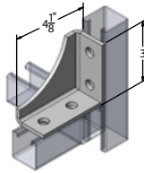
9033CA 4-hole webbed corner angle, l.h. 3-1/2" x 4-1/8"
