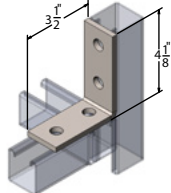
9030CA 4-hole corner angle 4-1/8" x 3-1/2"
