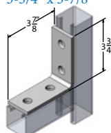
9031CA 4-hole corner angle 3-3/4" x 3-7/8"
